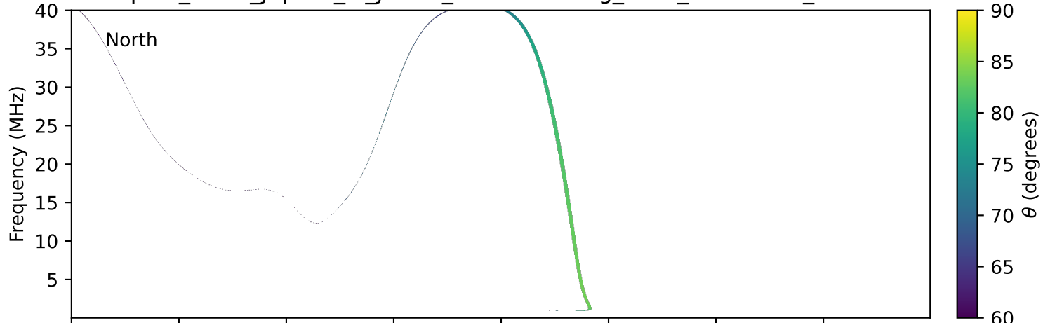
expres_earth_jupiter_io_jrm33_lossc-wid1deg_3kev_19960806_v11.cdf
