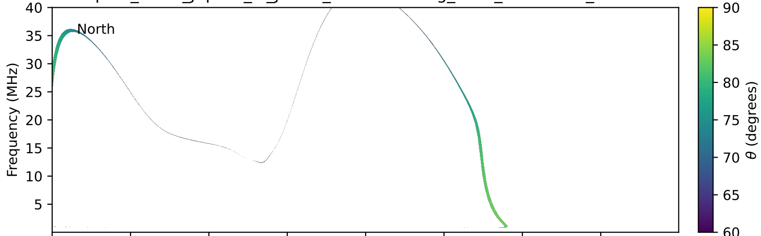
expres_earth_jupiter_io_jrm09_lossc-wid1deg_3kev_19960820_v11.cdf
