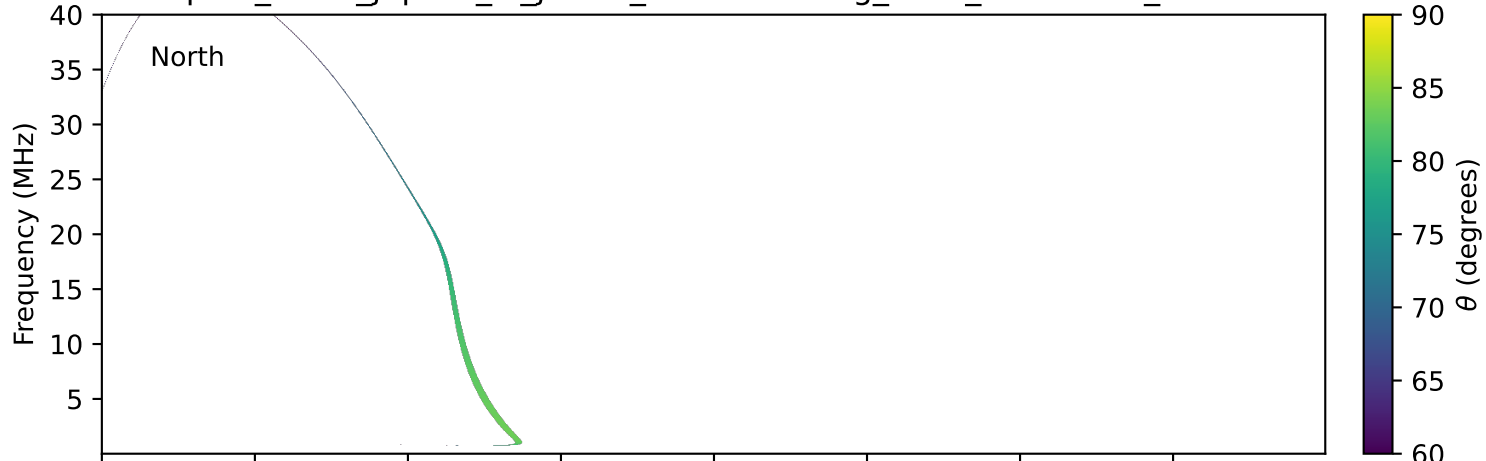
expres_earth_jupiter_io_jrm09_lossc-wid1deg_3kev_19960808_v11.cdf
