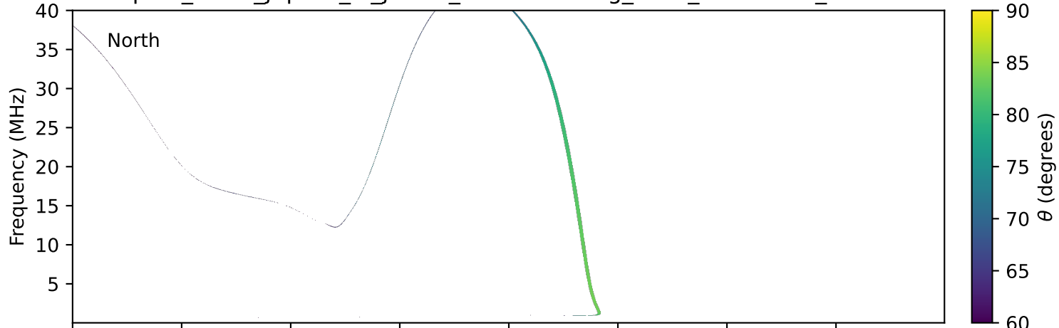
expres_earth_jupiter_io_jrm09_lossc-wid1deg_3kev_19960806_v11.cdf
