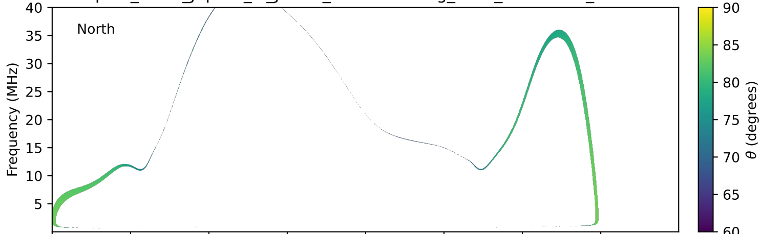
expres_earth_jupiter_io_jrm09_lossc-wid1deg_3kev_19960804_v11.cdf
