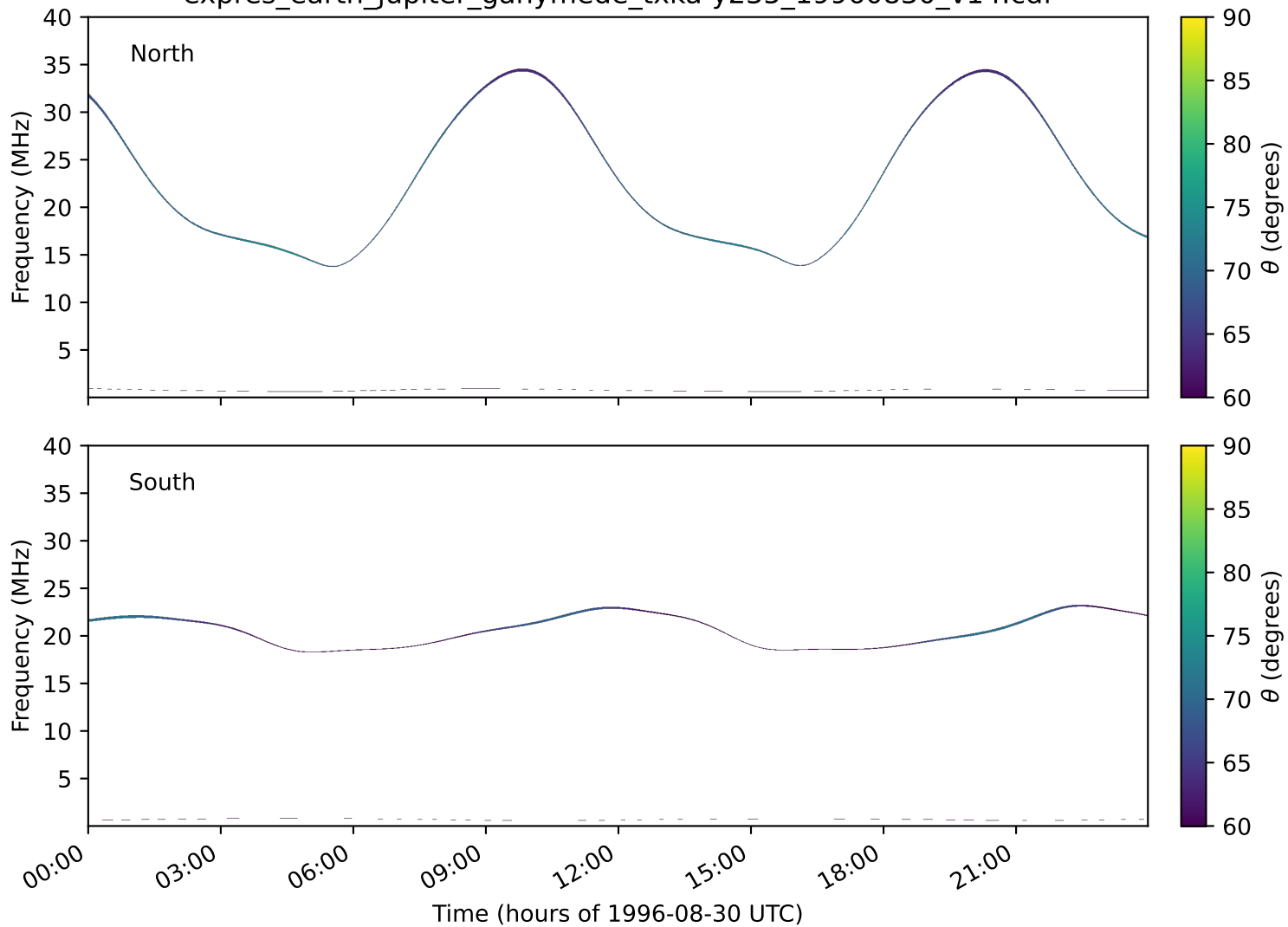
expres_earth_jupiter_ganymede_txka-y235_19960830_v14.cdf
