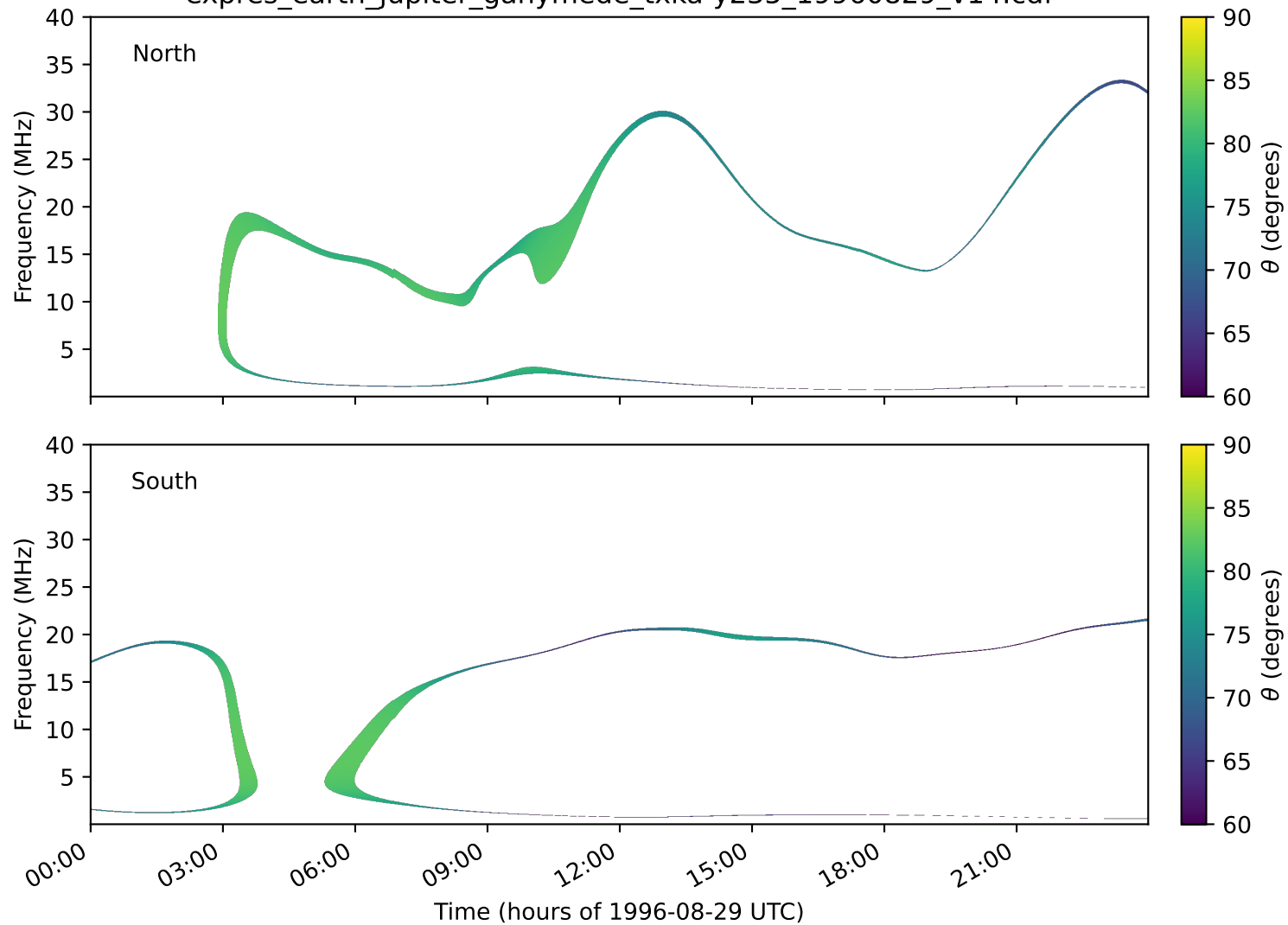
expres_earth_jupiter_ganymede_txka-y235_19960829_v14.cdf
