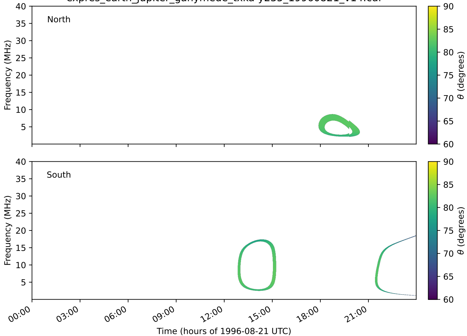
expres_earth_jupiter_ganymede_txka-y235_19960821_v14.cdf
