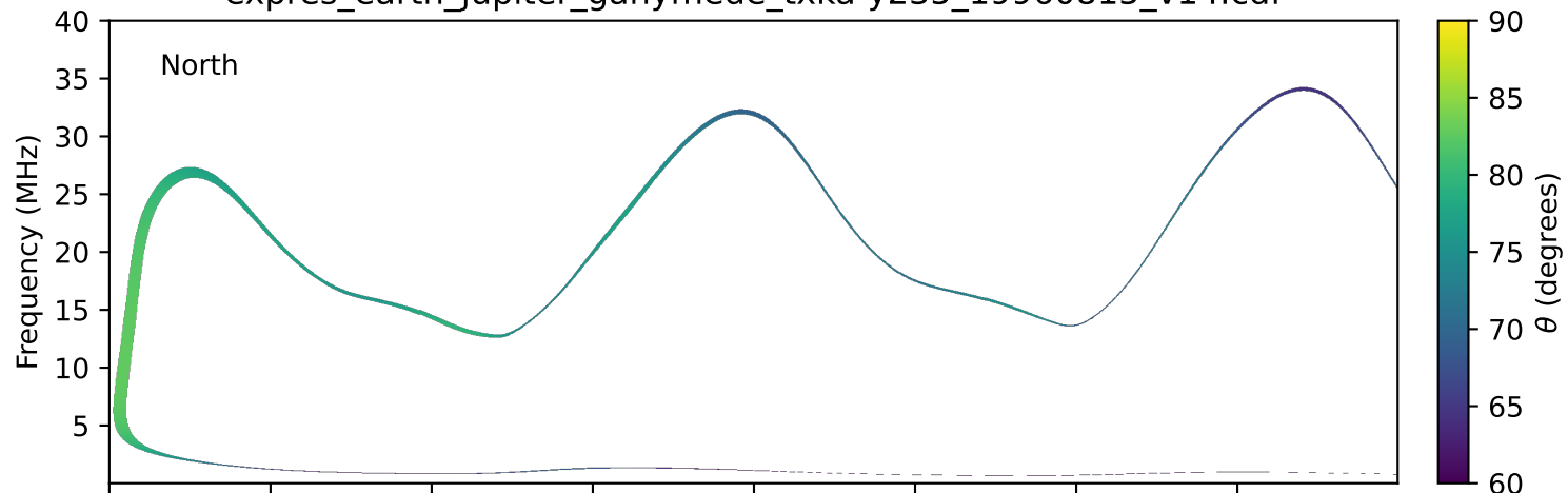
expres_earth_jupiter_ganymede_txka-y235_19960815_v14.cdf
