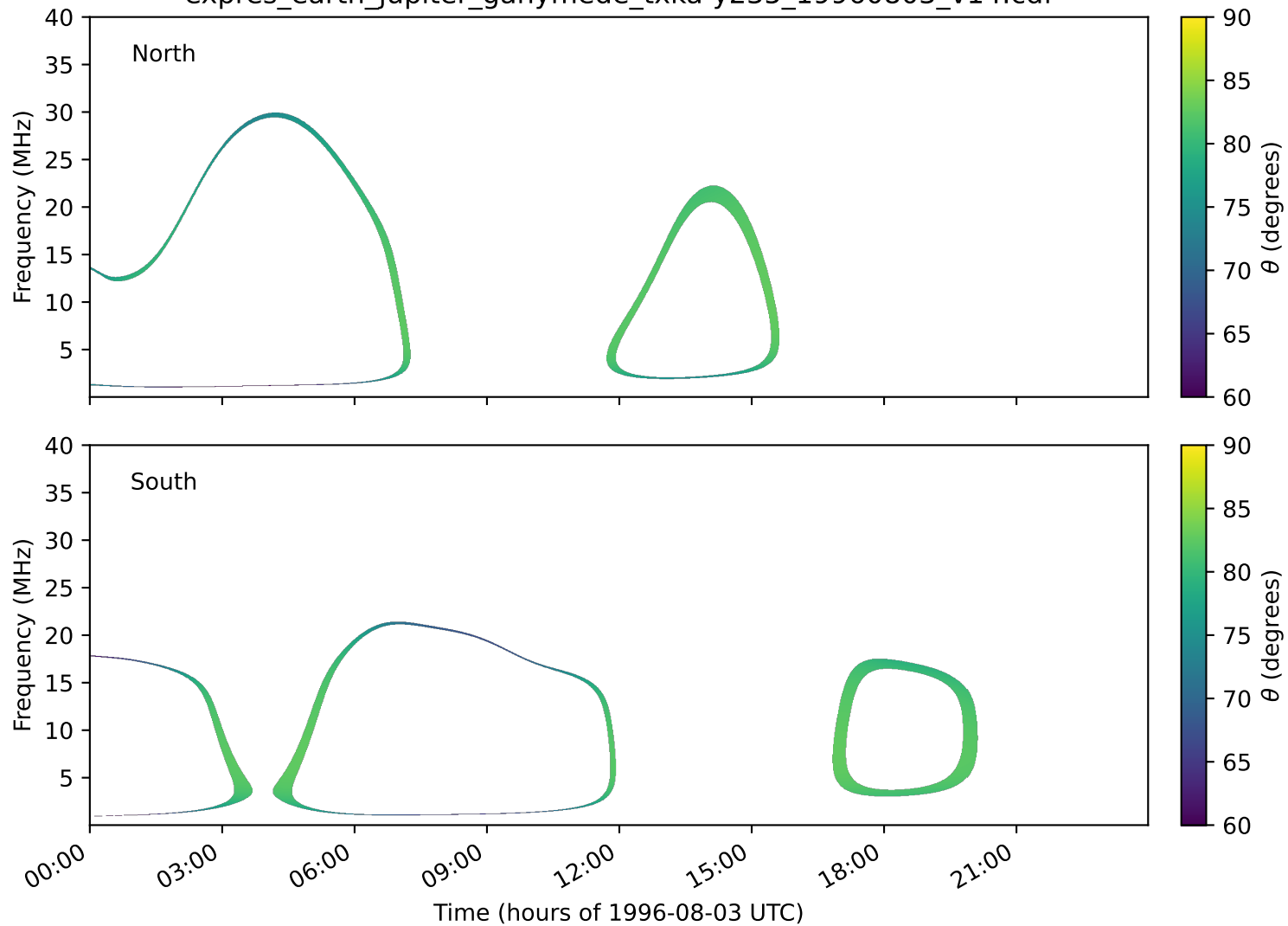
expres_earth_jupiter_ganymede_txka-y235_19960803_v14.cdf
