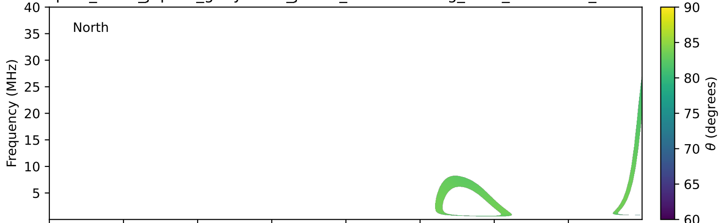
expres_earth_jupiter_ganymede_jrm33_lossc-wid1deg_3kev_19960807_v11.cdf
