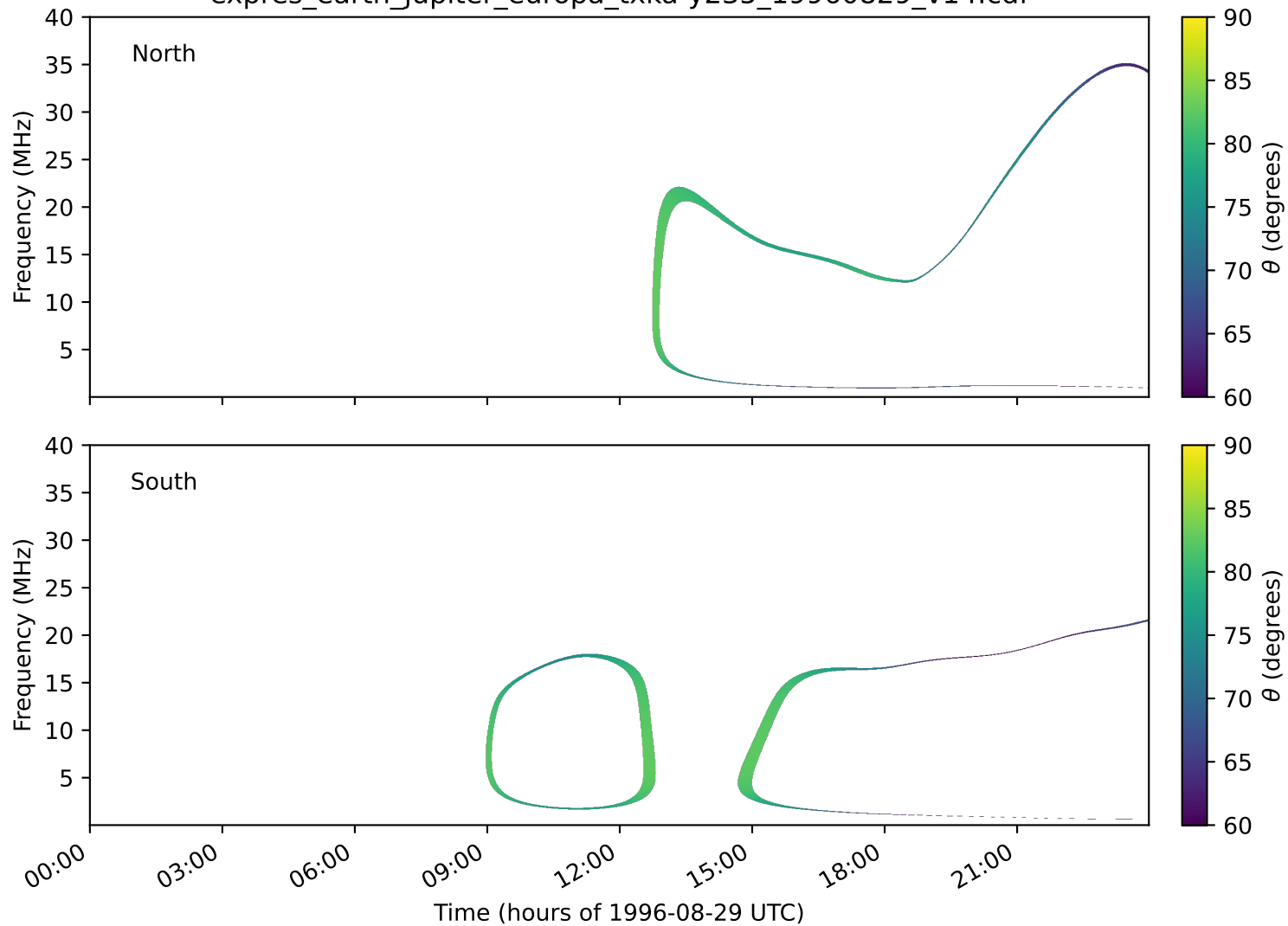
expres_earth_jupiter_europa_txka-y235_19960829_v14.cdf
