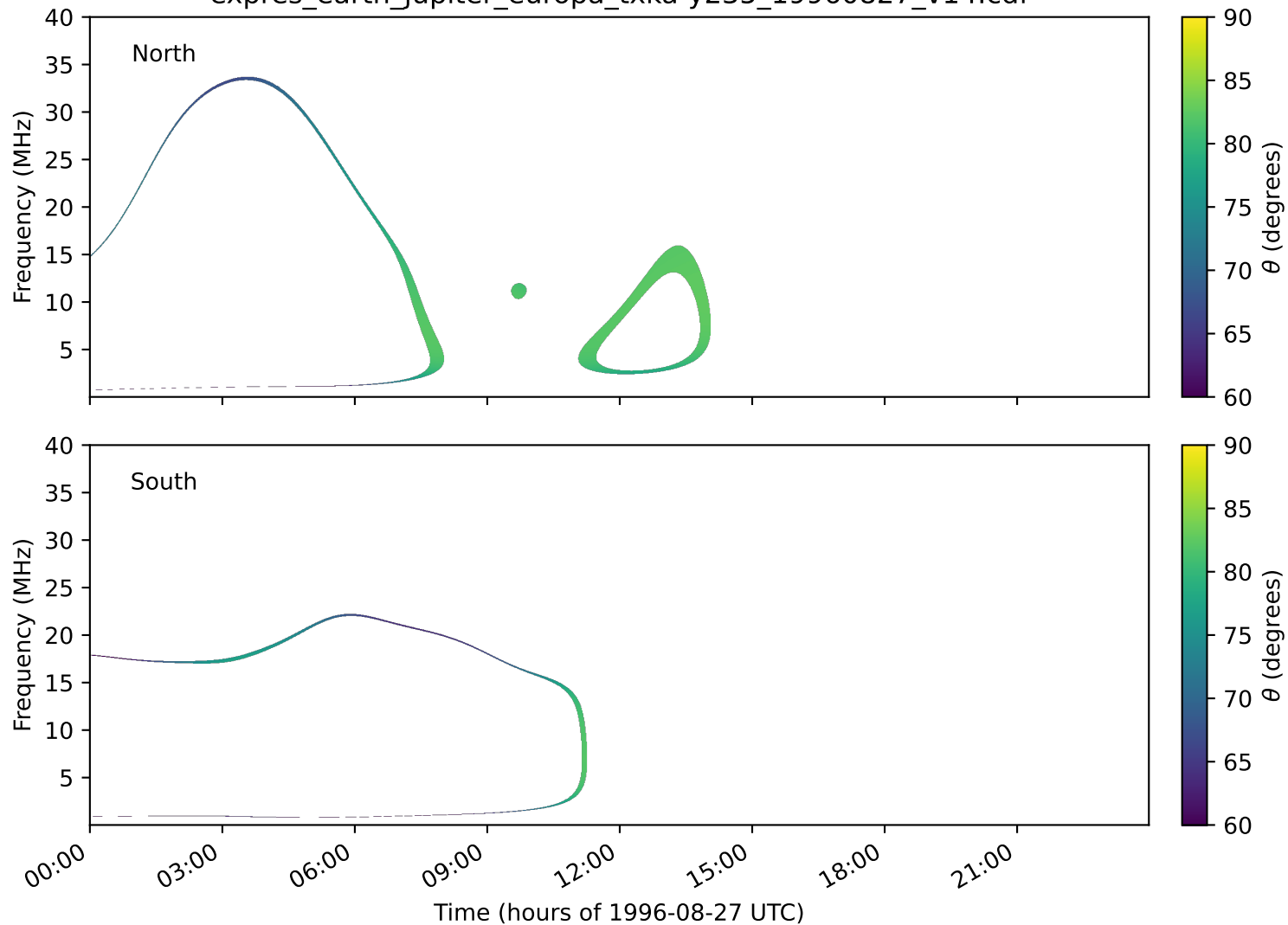
expres_earth_jupiter_europa_txka-y235_19960827_v14.cdf
