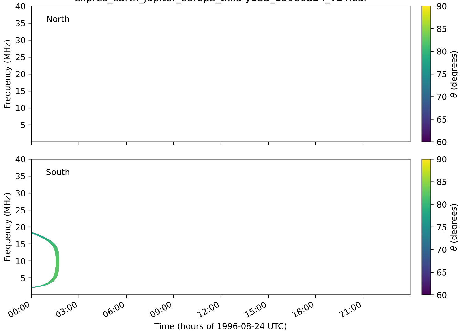
expres_earth_jupiter_europa_txka-y235_19960824_v14.cdf
