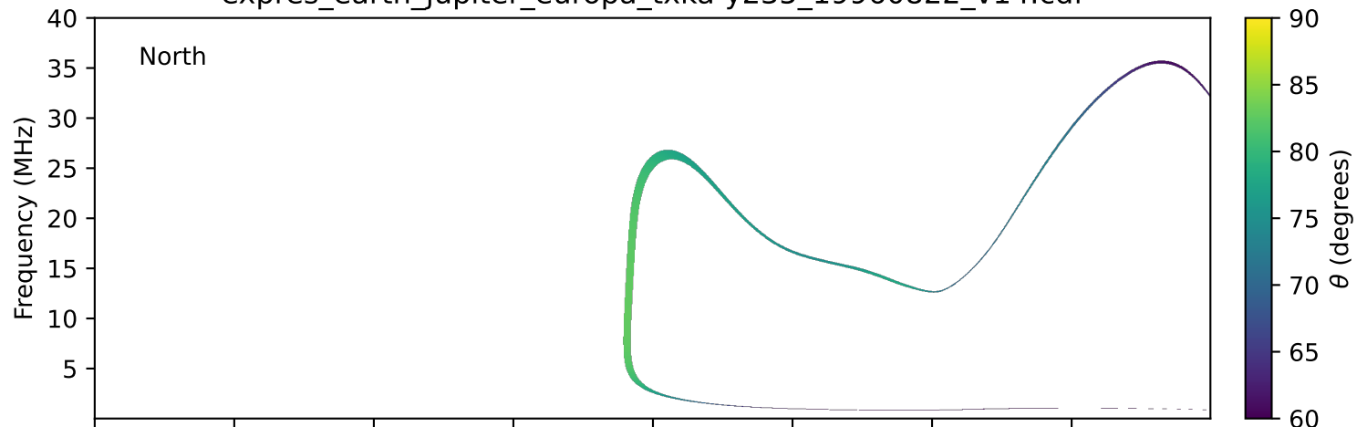
expres_earth_jupiter_europa_txka-y235_19960822_v14.cdf
