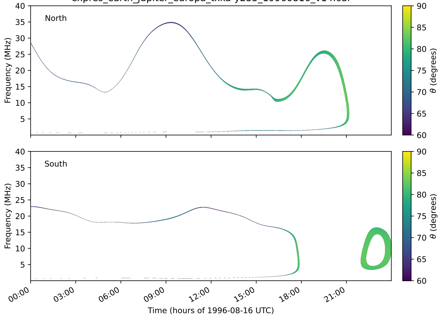
expres_earth_jupiter_europa_txka-y235_19960816_v14.cdf
