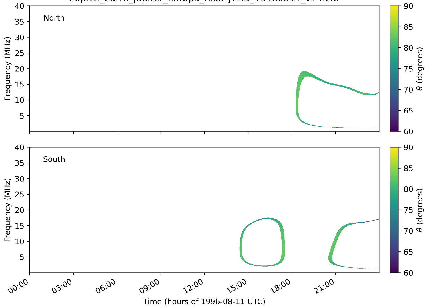
expres_earth_jupiter_europa_txka-y235_19960811_v14.cdf
