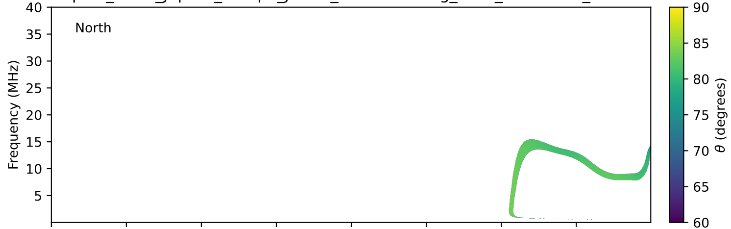
expres_earth_jupiter_europa_jrm33_lossc-wid1deg_3kev_19960811_v11.cdf
