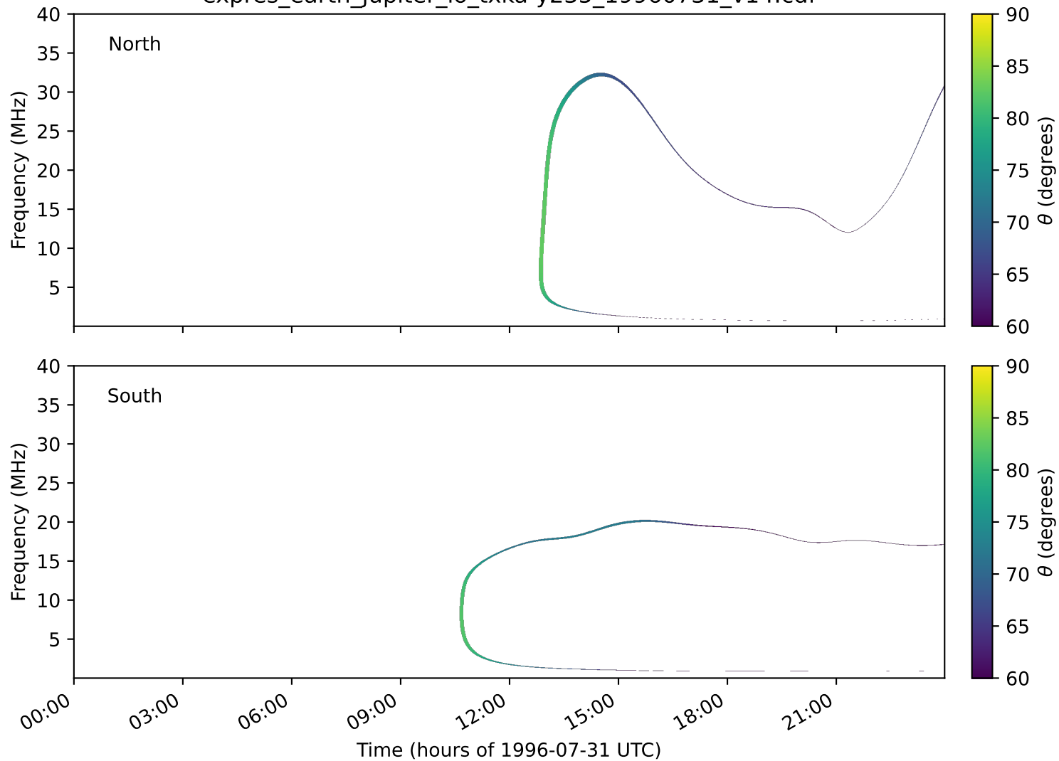
expres_earth_jupiter_io_txka-y235_19960731_v14.cdf
