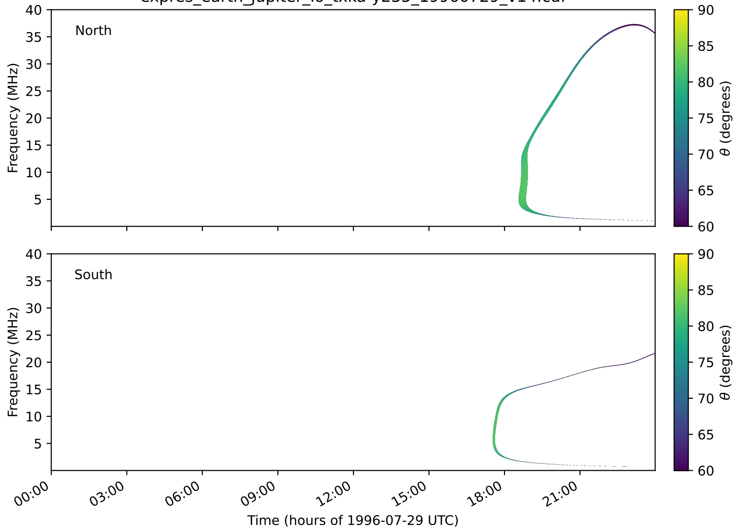
expres_earth_jupiter_io_txka-y235_19960729_v14.cdf
