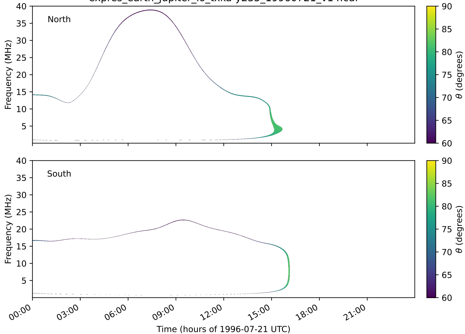
expres_earth_jupiter_io_txka-y235_19960721_v14.cdf
