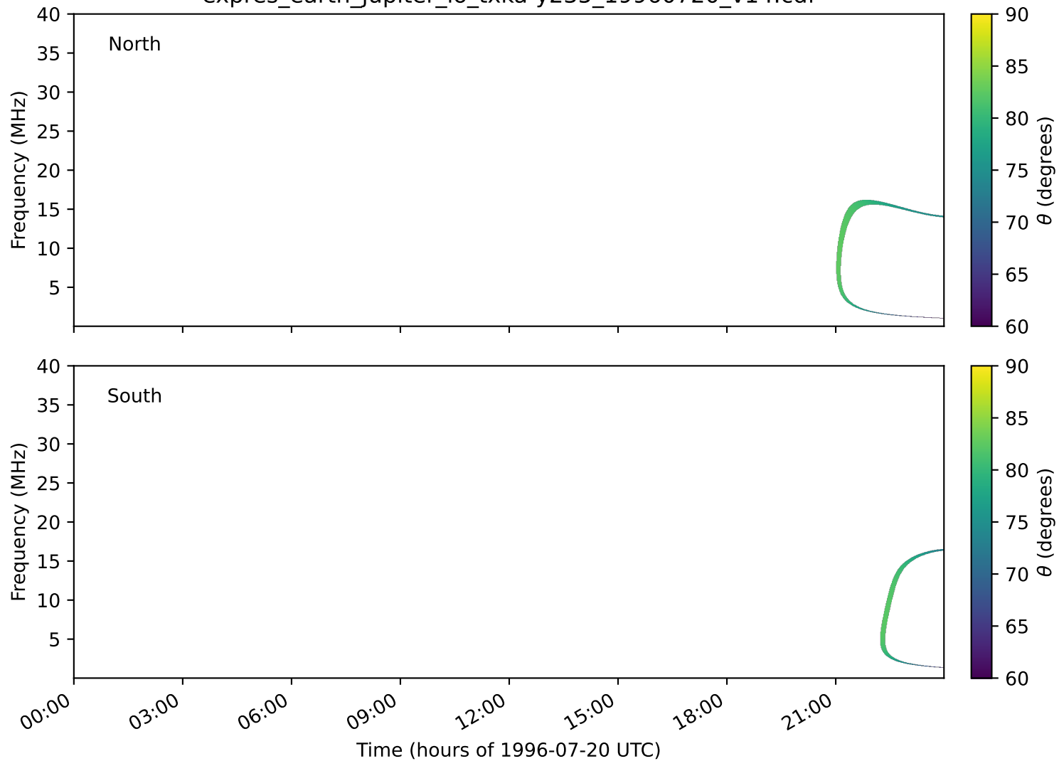
expres_earth_jupiter_io_txka-y235_19960720_v14.cdf
