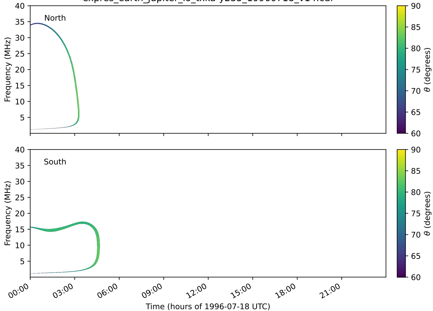
expres_earth_jupiter_io_txka-y235_19960718_v14.cdf
