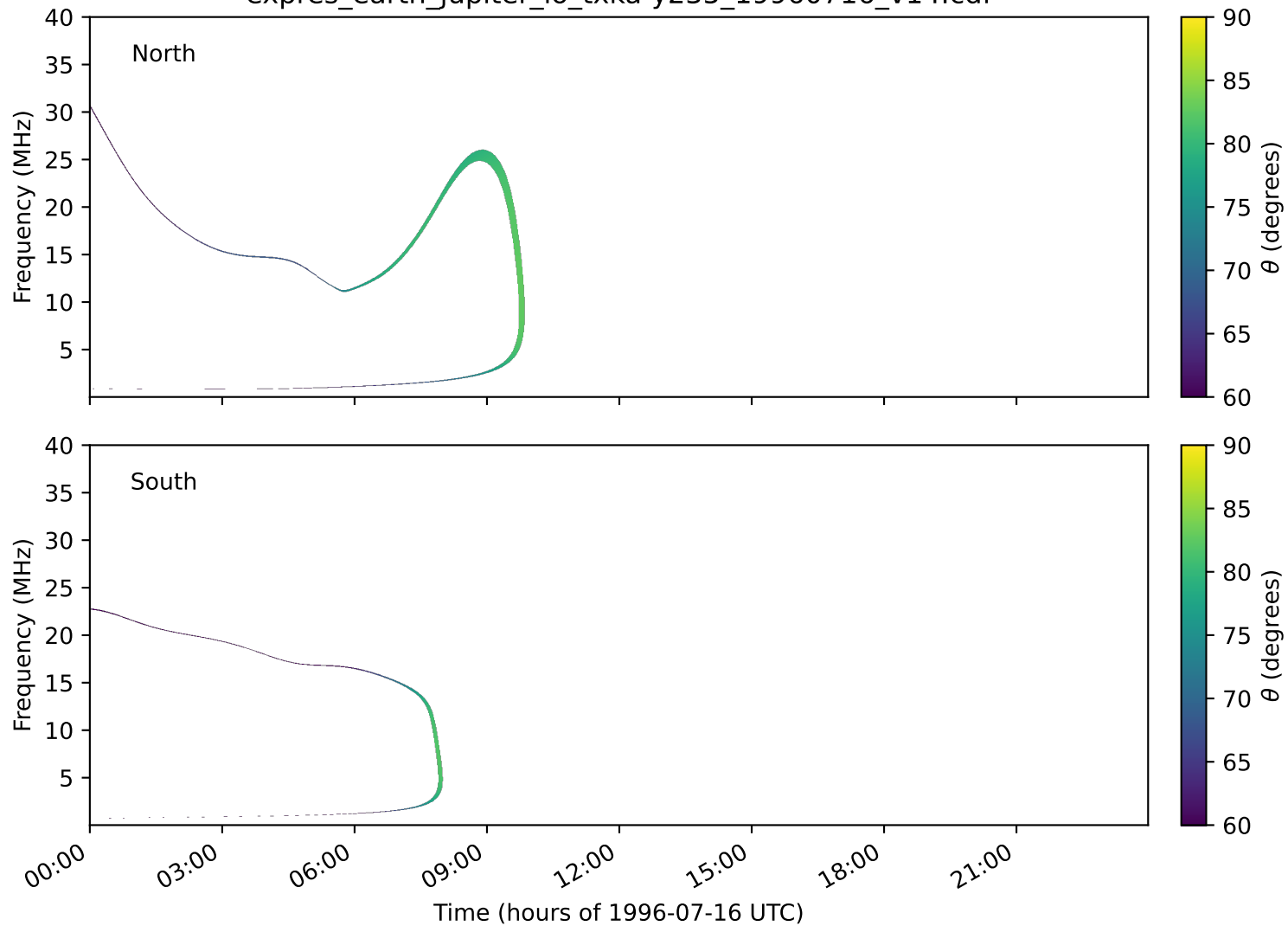
expres_earth_jupiter_io_txka-y235_19960716_v14.cdf
