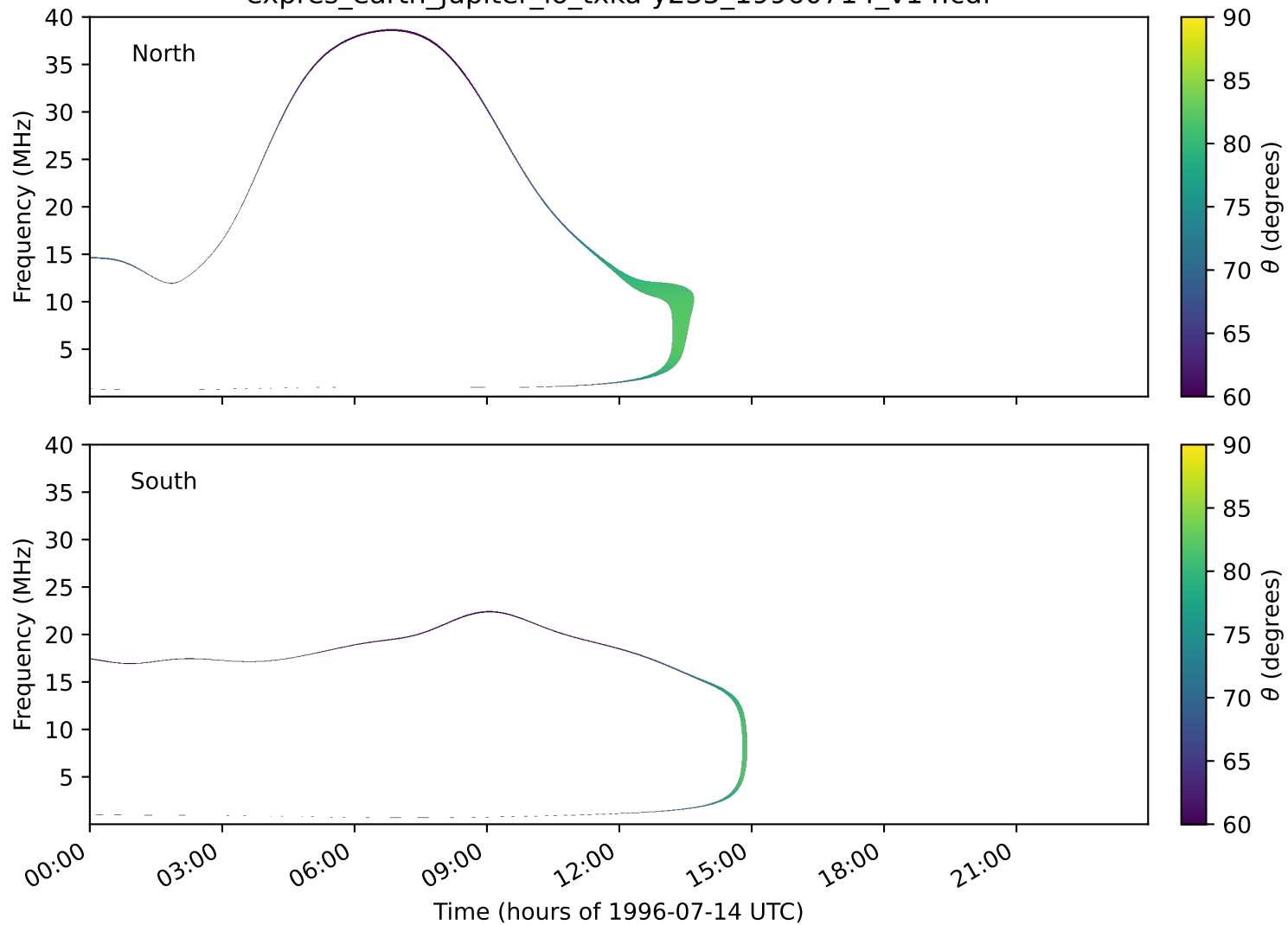
expres_earth_jupiter_io_txka-y235_19960714_v14.cdf
