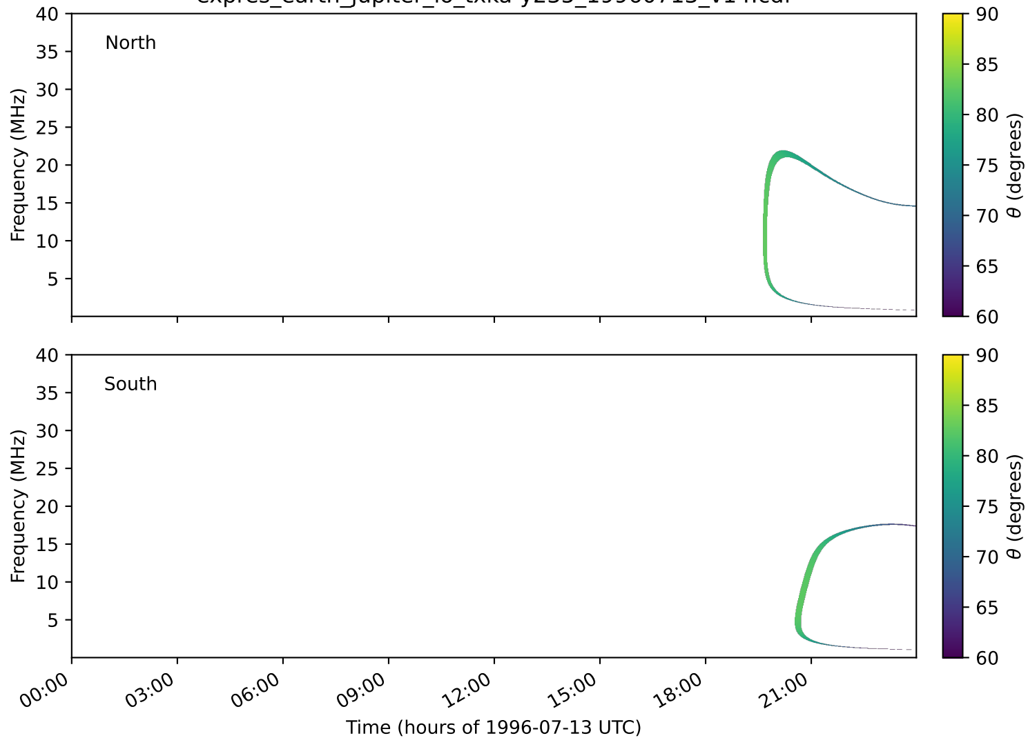
expres_earth_jupiter_io_txka-y235_19960713_v14.cdf
