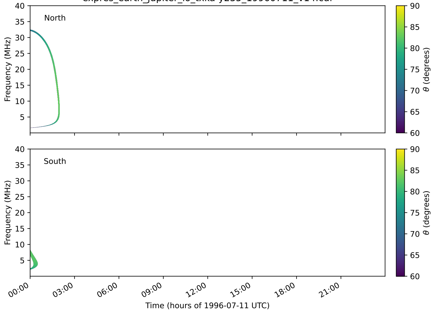
expres_earth_jupiter_io_txka-y235_19960711_v14.cdf
