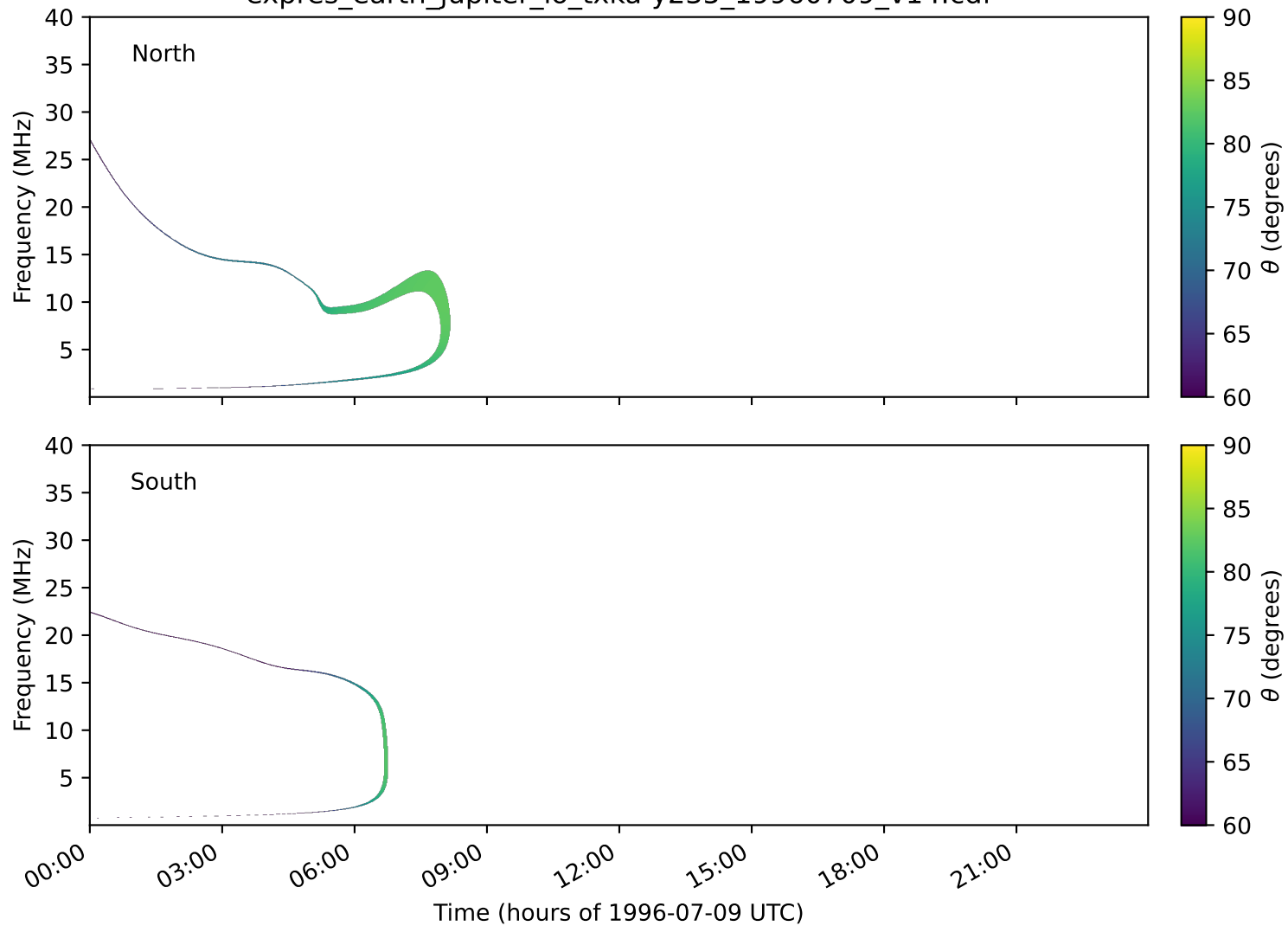
expres_earth_jupiter_io_txka-y235_19960709_v14.cdf
