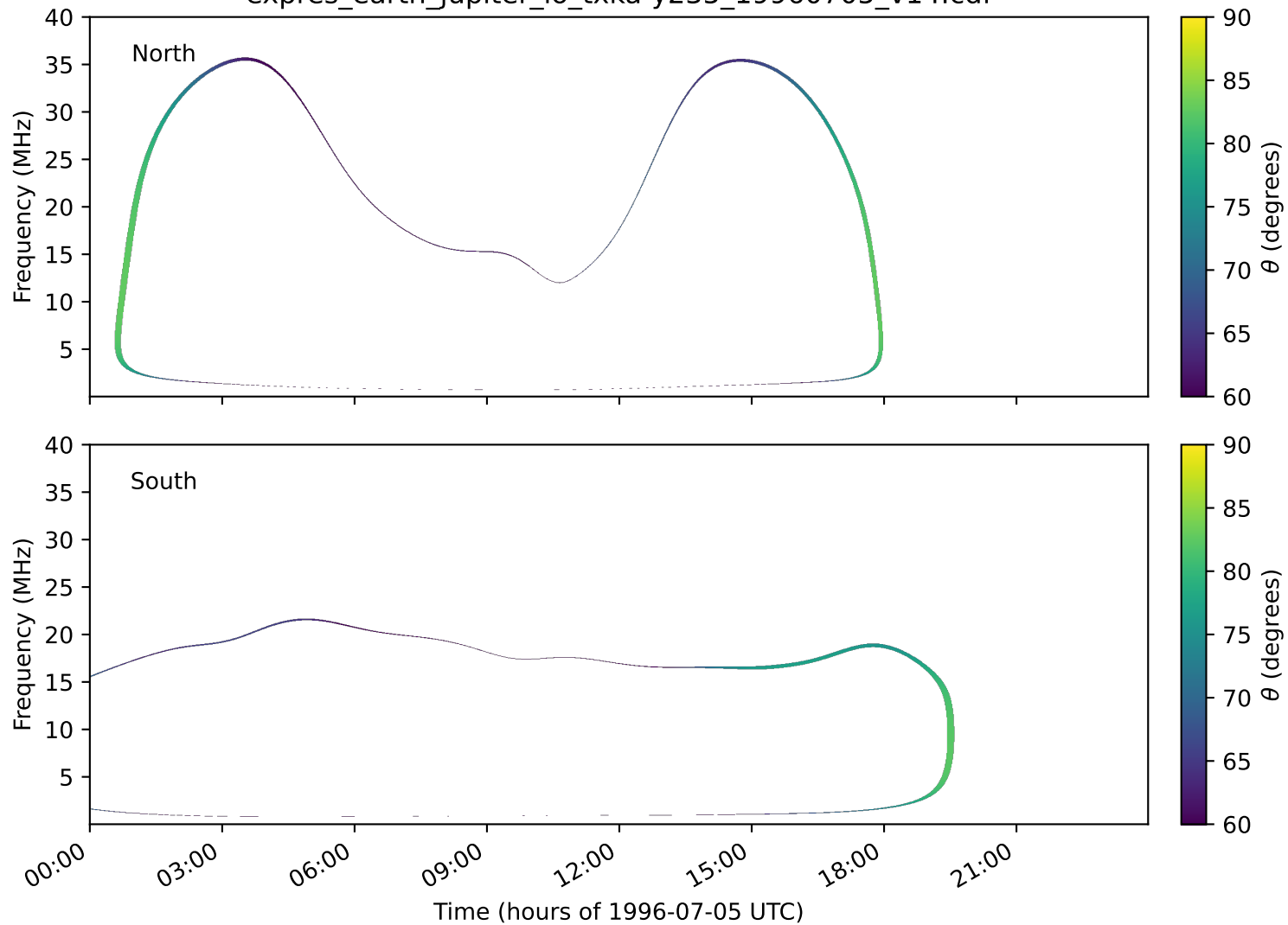
expres_earth_jupiter_io_txka-y235_19960705_v14.cdf
