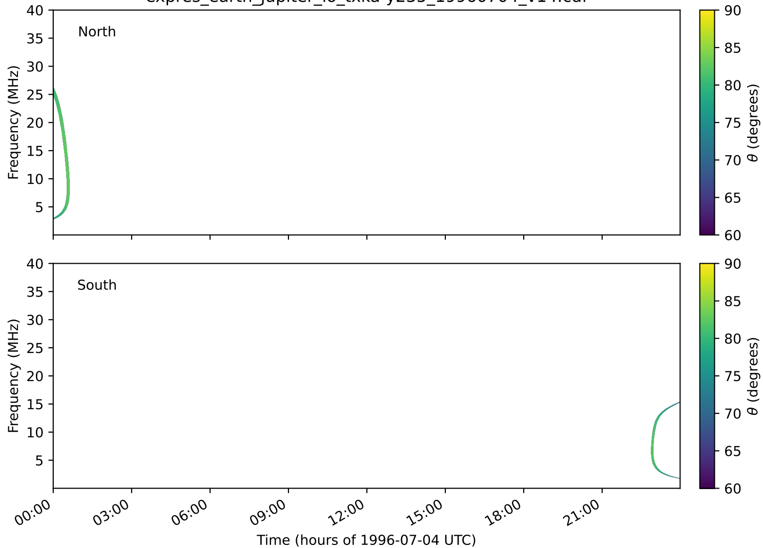
expres_earth_jupiter_io_txka-y235_19960704_v14.cdf
