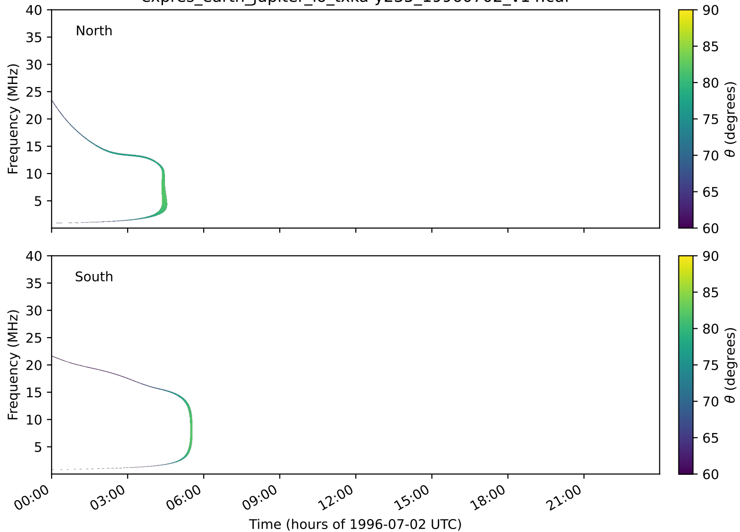
expres_earth_jupiter_io_txka-y235_19960702_v14.cdf
