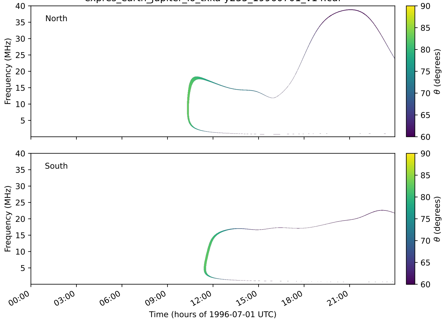
expres_earth_jupiter_io_txka-y235_19960701_v14.cdf
