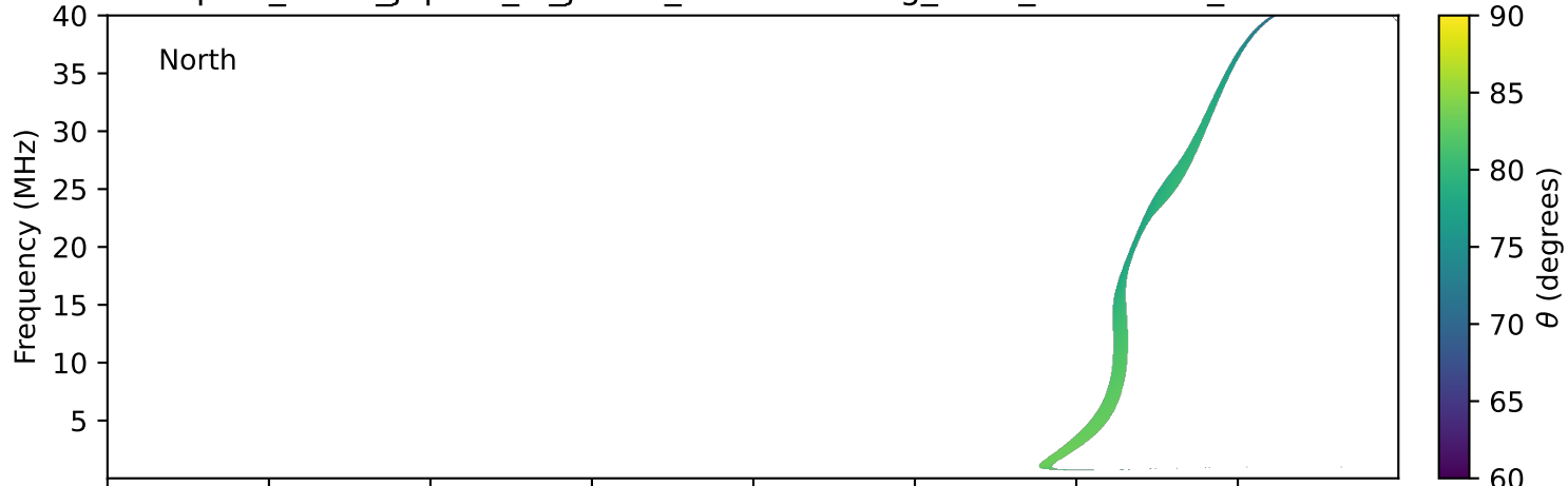
expres_earth_jupiter_io_jrm33_lossc-wid1deg_3kev_19960729_v11.cdf
