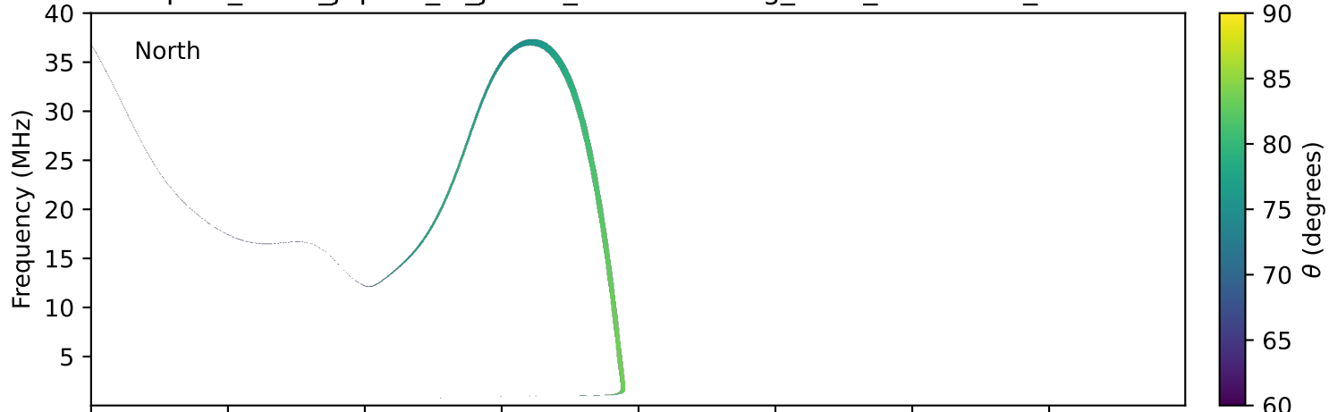
expres_earth_jupiter_io_jrm33_lossc-wid1deg_3kev_19960723_v11.cdf
