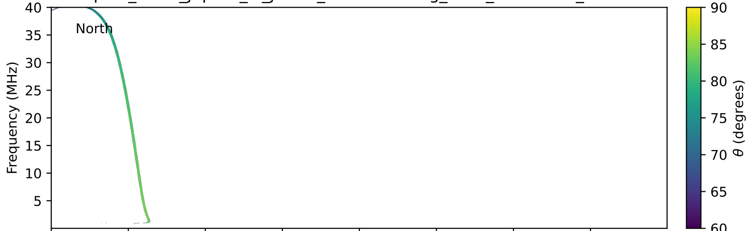
expres_earth_jupiter_io_jrm33_lossc-wid1deg_3kev_19960718_v11.cdf
