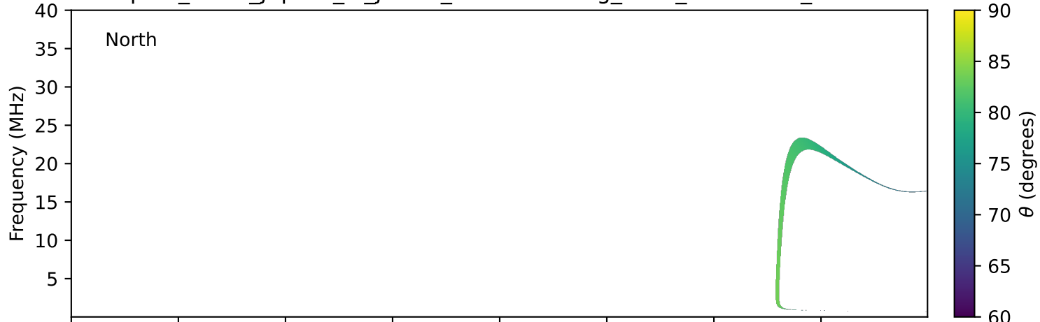
expres_earth_jupiter_io_jrm33_lossc-wid1deg_3kev_19960713_v11.cdf
