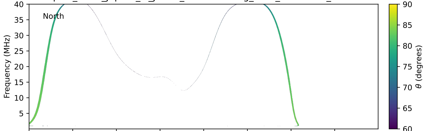
expres_earth_jupiter_io_jrm33_lossc-wid1deg_3kev_19960705_v11.cdf
