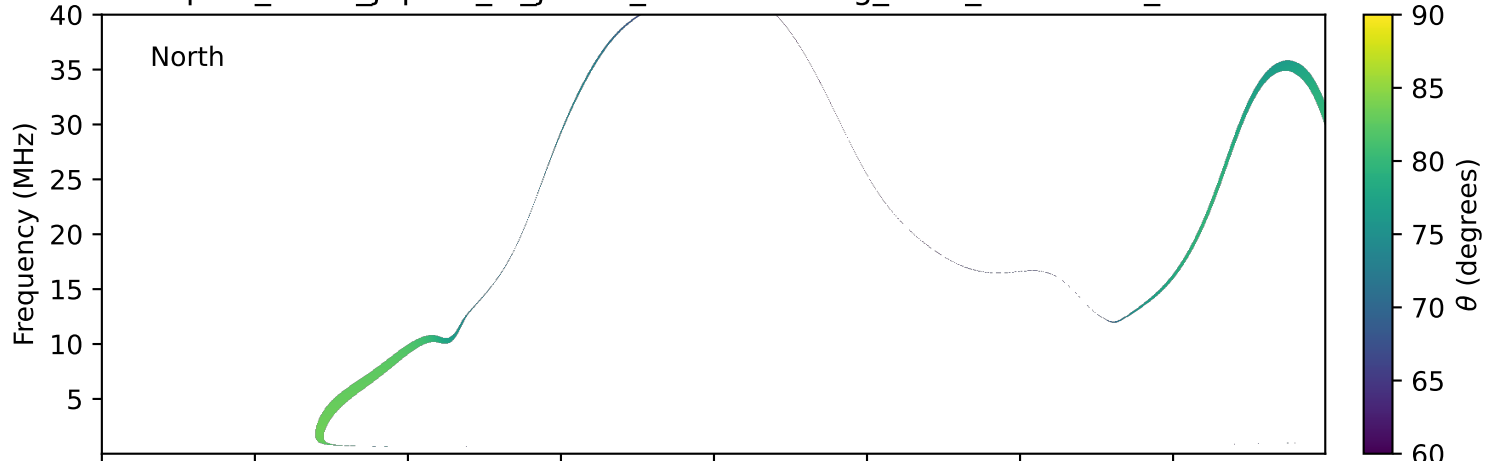
expres_earth_jupiter_io_jrm33_lossc-wid1deg_3kev_19960703_v11.cdf
