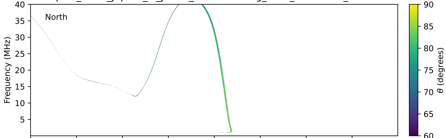
expres_earth_jupiter_io_jrm09_lossc-wid1deg_3kev_19960730_v11.cdf
