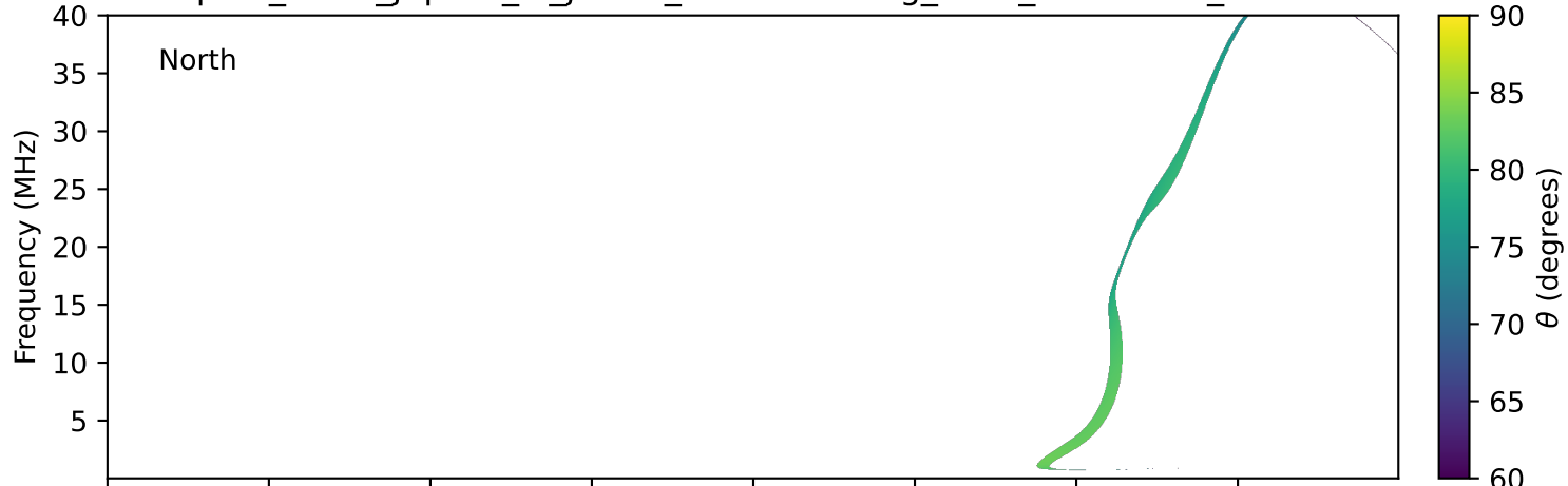
expres_earth_jupiter_io_jrm09_lossc-wid1deg_3kev_19960729_v11.cdf
