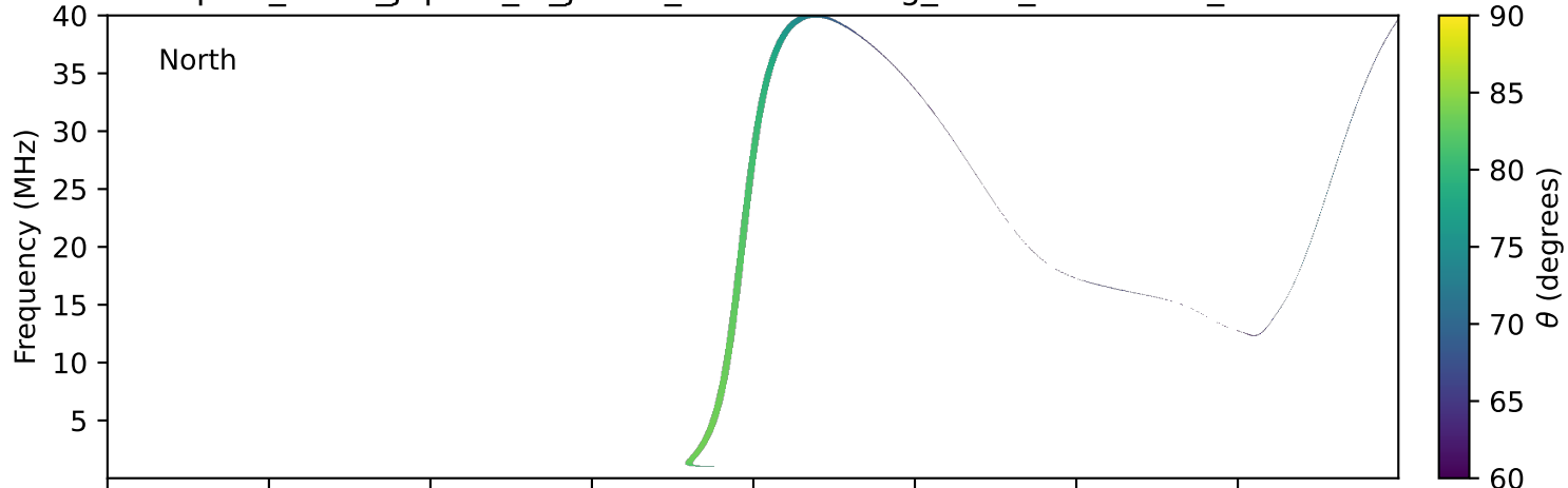
expres_earth_jupiter_io_jrm09_lossc-wid1deg_3kev_19960724_v11.cdf
