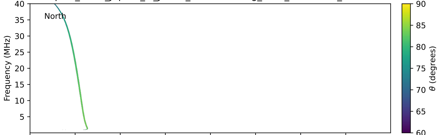
expres_earth_jupiter_io_jrm09_lossc-wid1deg_3kev_19960718_v11.cdf
