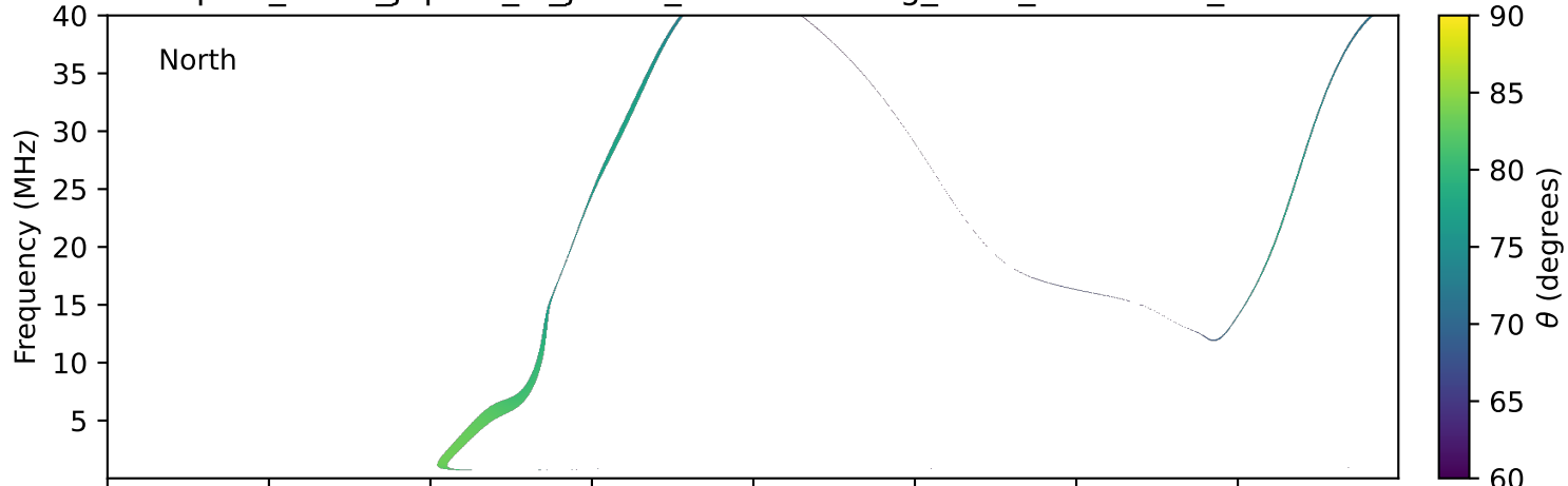
expres_earth_jupiter_io_jrm09_lossc-wid1deg_3kev_19960710_v11.cdf
