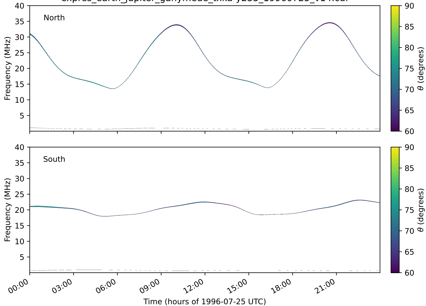
expres_earth_jupiter_ganymede_txka-y235_19960725_v14.cdf
