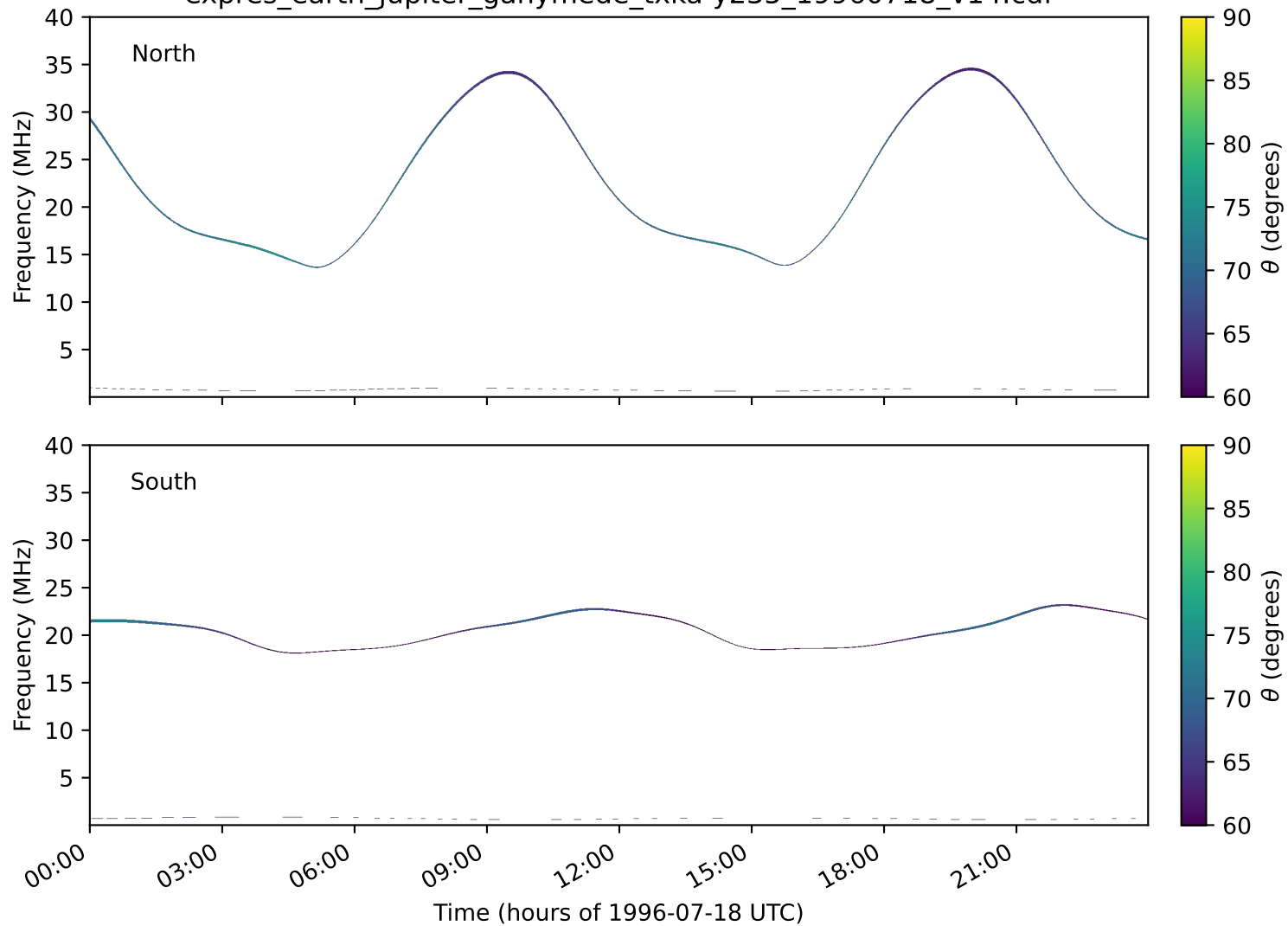
expres_earth_jupiter_ganymede_txka-y235_19960718_v14.cdf
