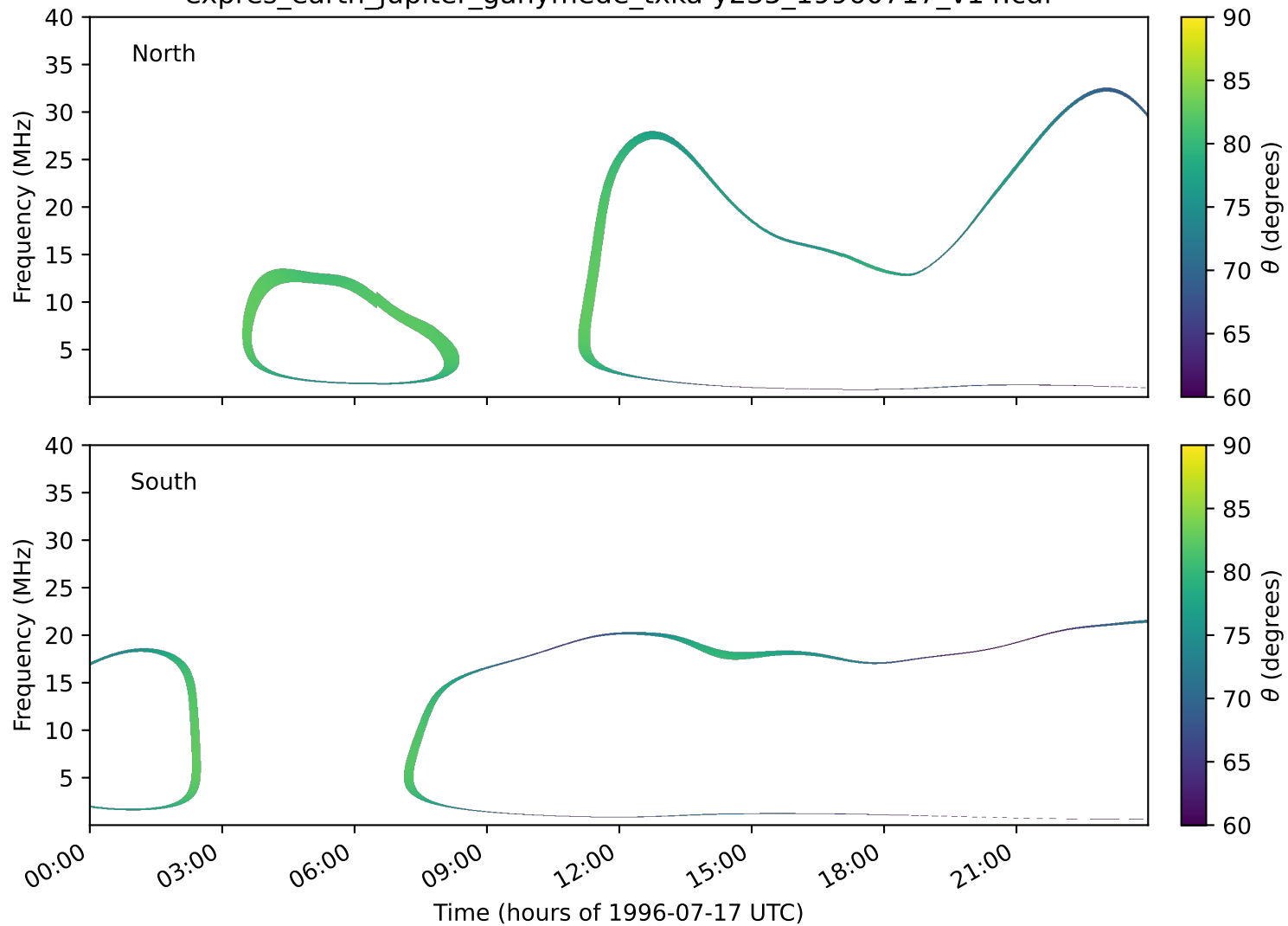
expres_earth_jupiter_ganymede_txka-y235_19960717_v14.cdf
