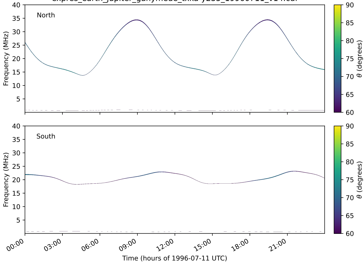
expres_earth_jupiter_ganymede_txka-y235_19960711_v14.cdf
