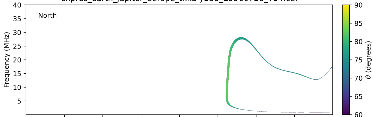
expres_earth_jupiter_europa_txka-y235_19960728_v14.cdf
