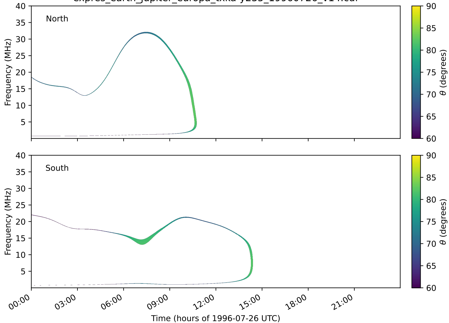
expres_earth_jupiter_europa_txka-y235_19960726_v14.cdf
