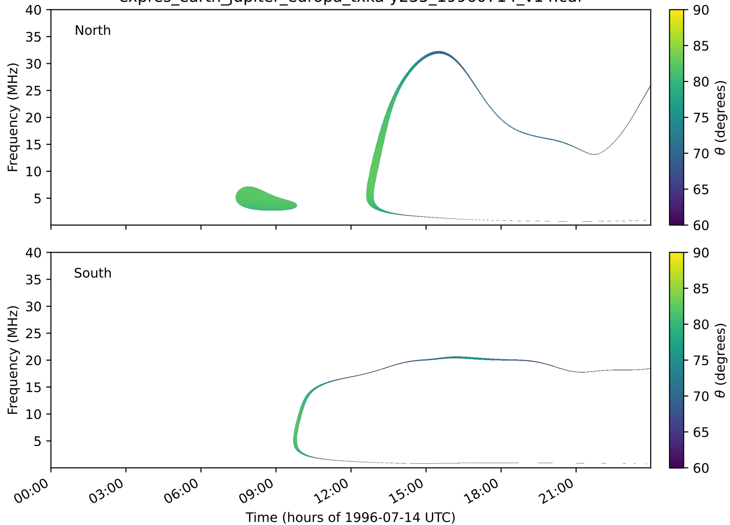
expres_earth_jupiter_europa_txka-y235_19960714_v14.cdf
